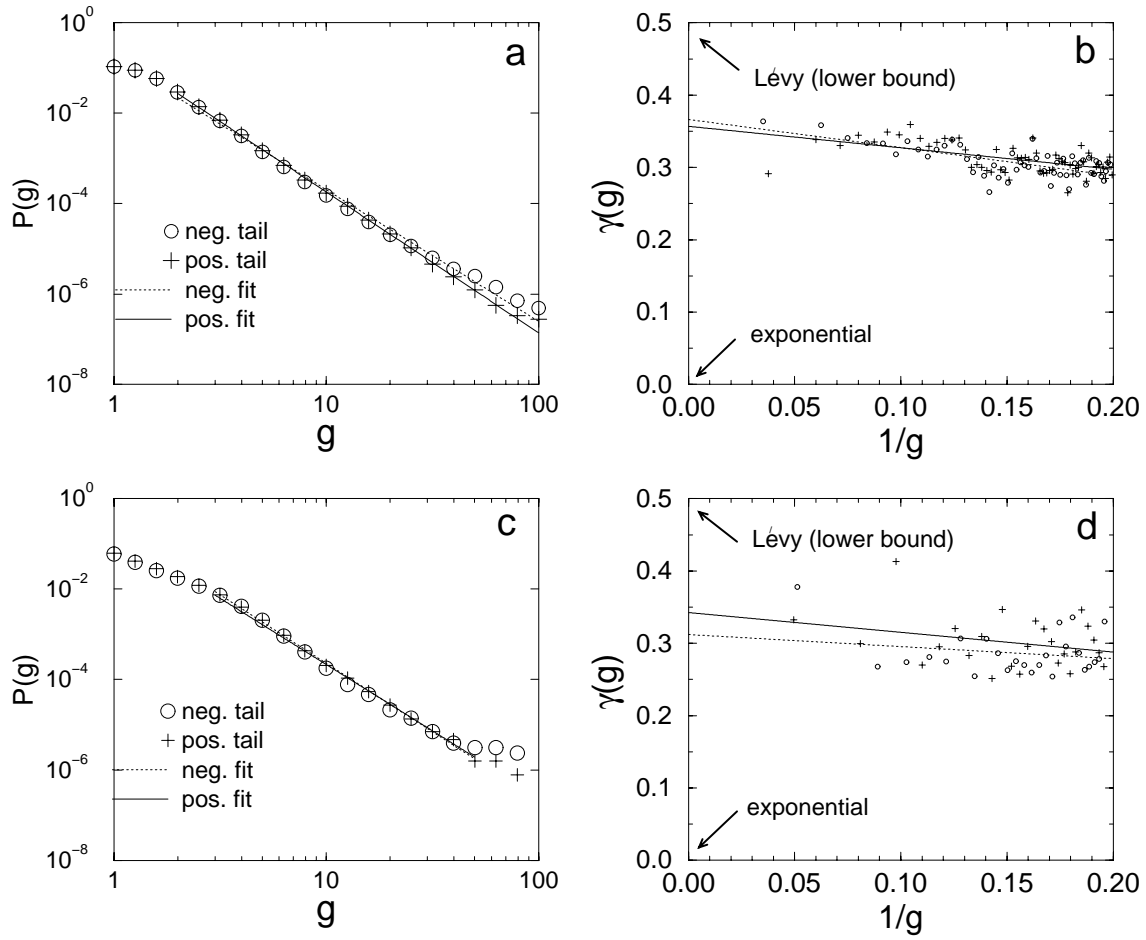
Fig. 1. (a) Log-log plot of the cumulative probability distribution P(g) of the normalized price increments g_i(t) . The lines in (a) are power law fits to the data over the range 2 < g < 100 . (b) The inverse local slope of P(g) , \gamma(g) \equiv -(d \log P(g)/d \log g)^{-1} as a function of 1/g for the negative ( \circ ) and the positive ( + ) tail respectively. We obtain an estimator for \gamma(g) , by sorting the normalized increments by their size, g^{(1)} > g^{(2)} > \dots > g^{(N)} . The cumulative density can then be written as P(g^{(k)}) = k/N , and we obtain for the local slope \gamma(g^{(k)}) = -\log(g^{(k+1)}/g^{(k)})/\log(P(g^{(k+1)})/P(g^{(k)})) \simeq k(\log(g^{(k+1)}) - \log(g^{(k)})) . Each data point shown in b is an average over 1000 increments g^{(k)} , and the lines are linear regression fits to the data. Note that the average m^{-1} \sum_{k=1}^m \gamma(g^{(k)}) over all events used would be identical to the estimator for the asymptotic slope proposed by Hill [9]. (c) Same as (a) for the 1 min S&P500 increments. The regression lines yield \alpha = 2.93 and \alpha = 3.02 for the positive and negative tails respectively. (d) Same as (b) for the 1 min S&P500 increments, except that the number of increments per data point is 100.
